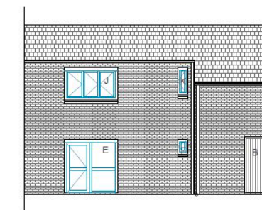
FACADE ARRIERE- T5
