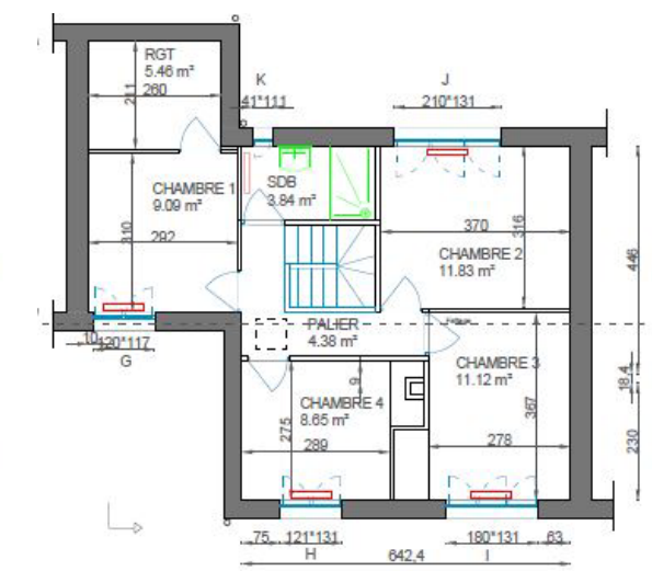
PLAN R+1 - T5
